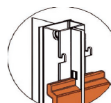
ADS with Open Joint Profile (ADS odprti fugni profil)
