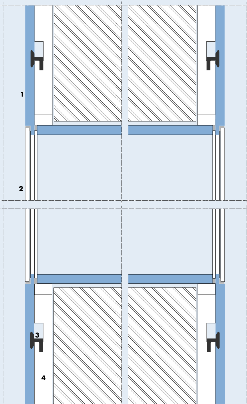
Vertical cross-section
