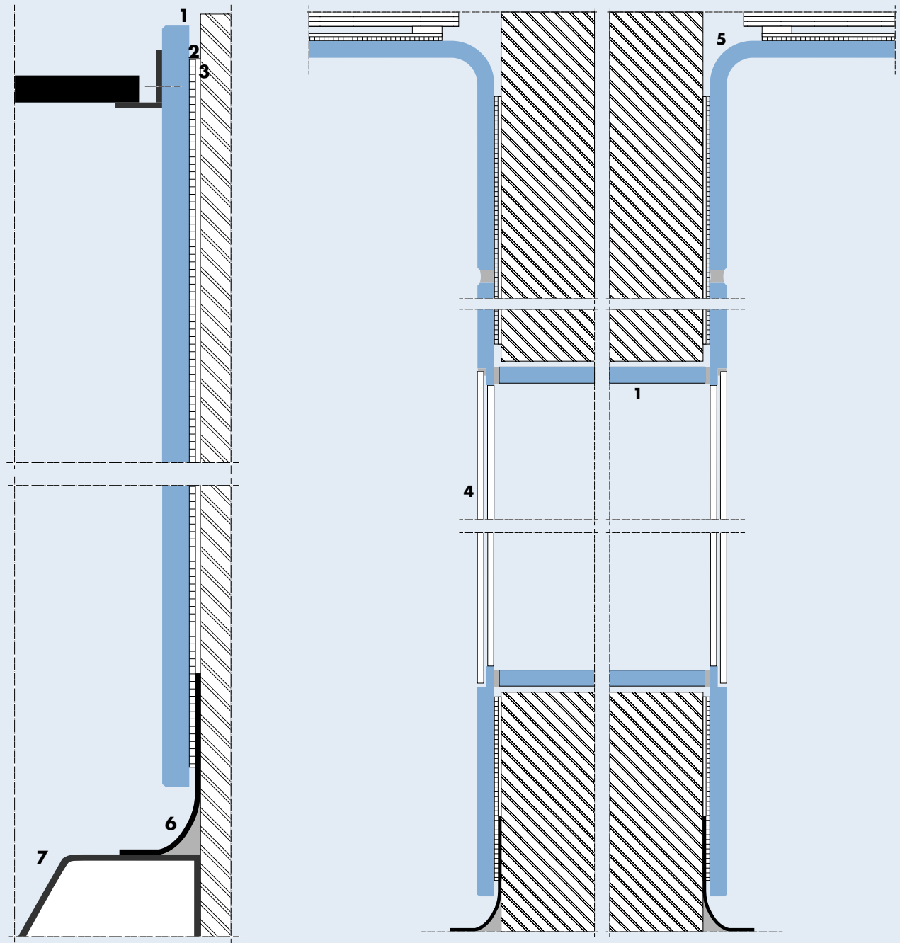
Vertical cross-section
