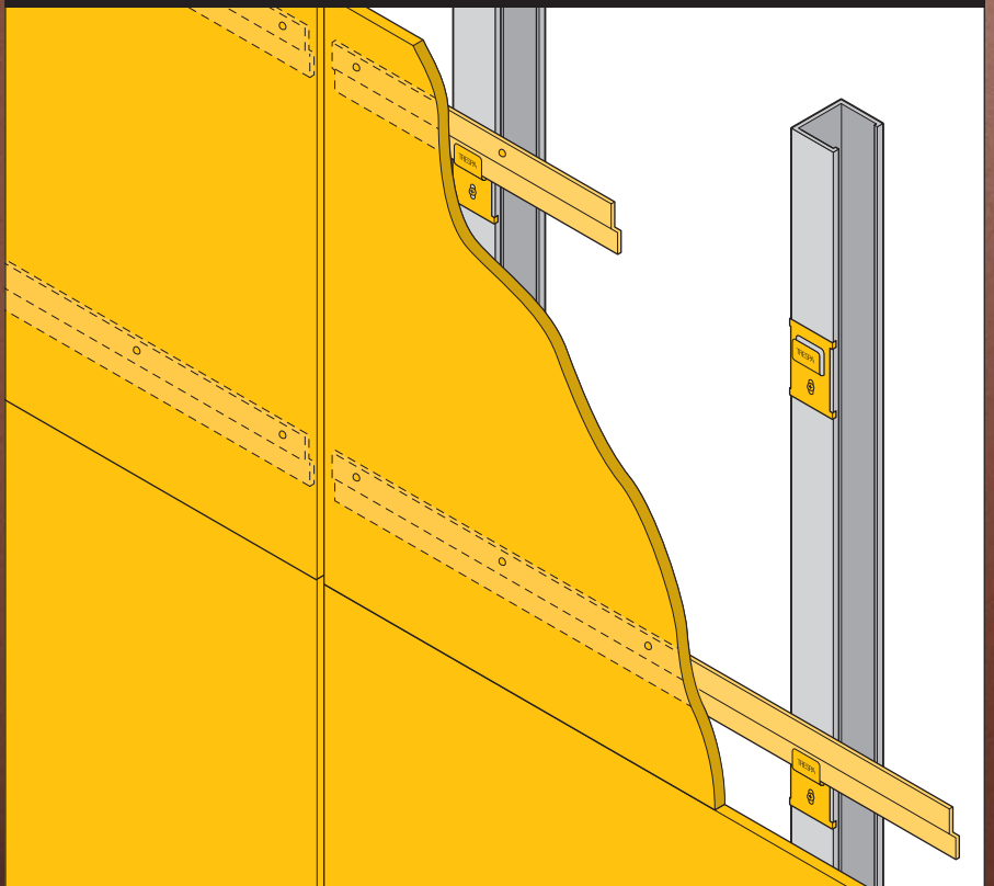
Trespa panel with z-profile clipped onto a metal framework
