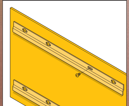
Z-profile fixed on Trespa panel
